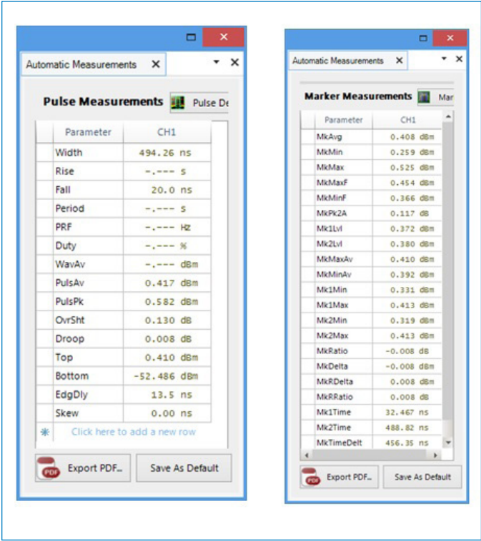
Figure 4. Automated Pulse & Marker Measurements using RTP5000 Series Real-Time Peak Power Sensors
