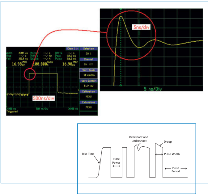
Figure 5. Some of the pulse characteristics that can be measured using a peak power meter.
