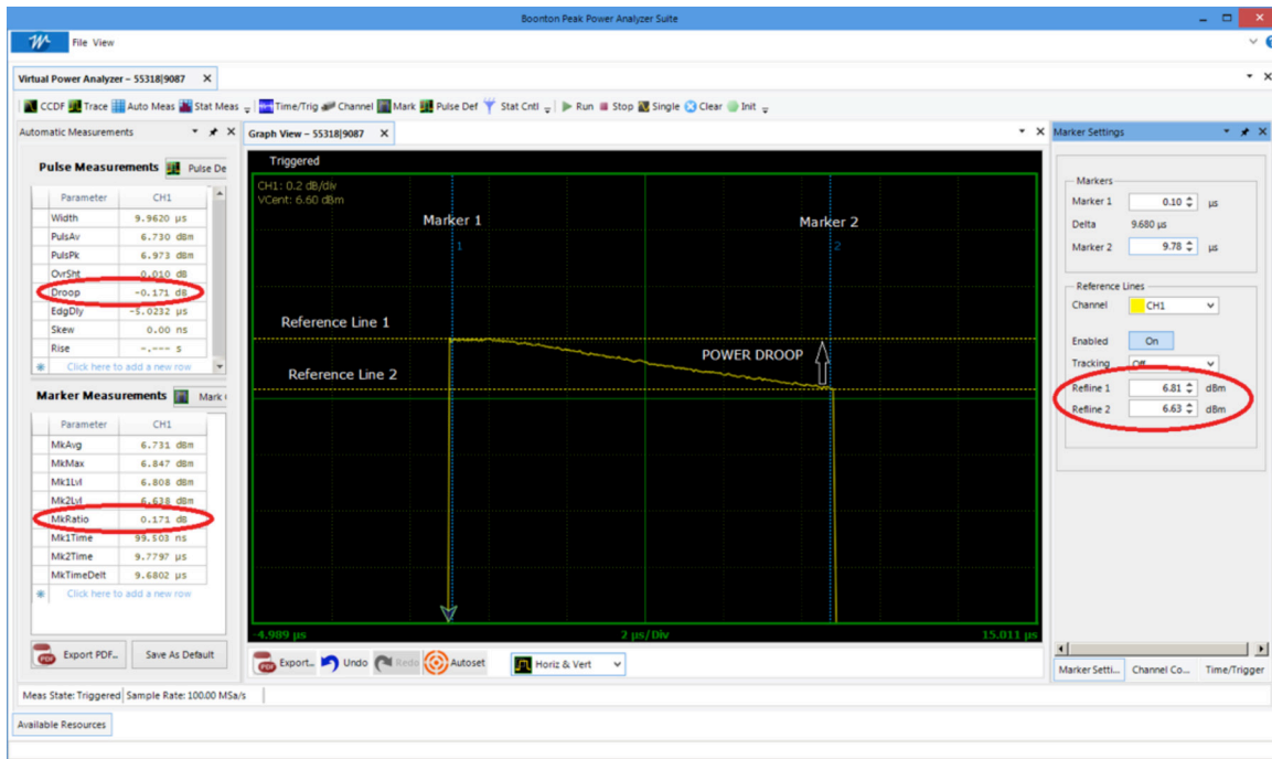
Figure 9. Droop Measurement using RTP5318 Real-Time Peak Power Sensors. Blue vertical lines 1 and 2 are markers placed for automated marker measurements. Yellow dashed horizontal lines are reference lines. Automated Pulse measurements are computed automatically based on pulse definition irrespective of marker or reference line placements.
