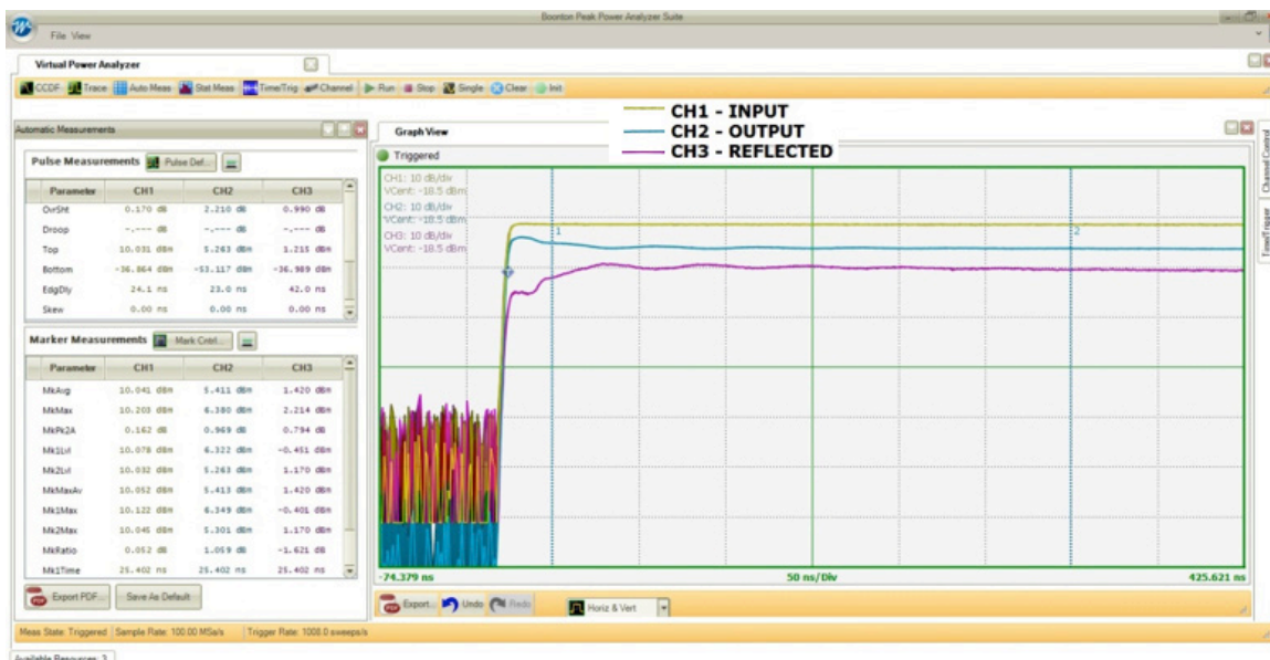
Figure 8. The screenshot captures the input, output and reflected waveforms of the pulsed RF signal. Blue trace is output of the DUT1 (note overshoot and ringing), purple trace is the reflect signal from the input port of the load DUT2.
