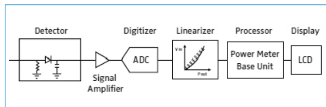
Figure 1. Peak Power Meter Block Diagram
