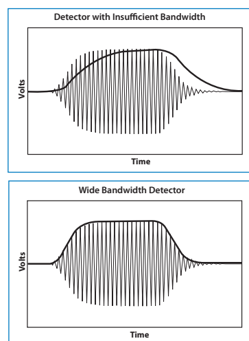
Figure 2. Impact of risetime and bandwidth capability of the sensor for accurately measuring and displaying the pulse RF signal.
